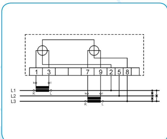
3u – three-phase, three wires, balanced load
