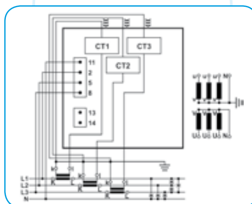
4u – four-wire, unbalanced load
