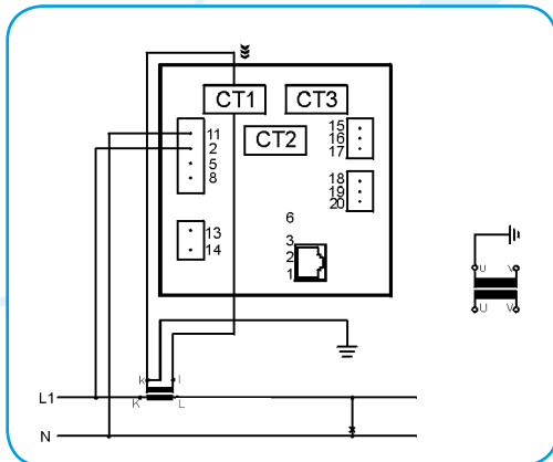
1b - single phase, balanced load
