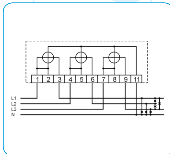
4u – three-phase, four wires, unbalanced load
