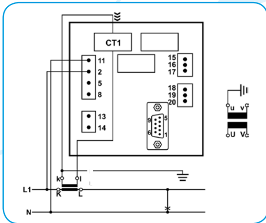
1b - single wire, balanced load
