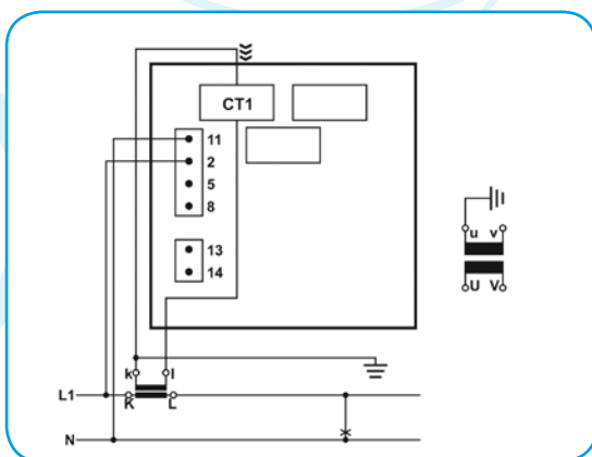
1b – single-wire, balanced load
