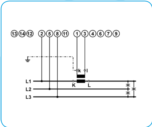
3b – three-phase, three wires, balanced load
