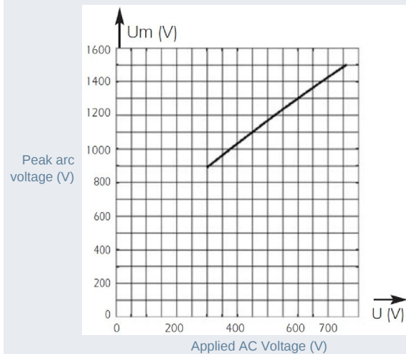
Peak arc voltage Size 00
