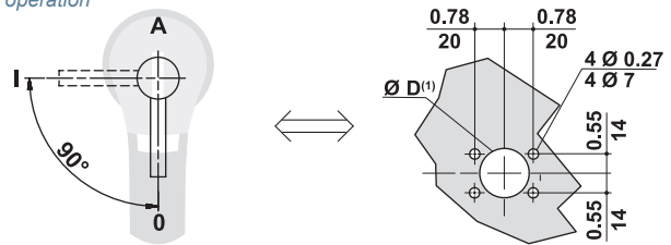
Front operation
