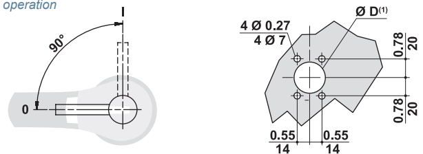
Side operation
